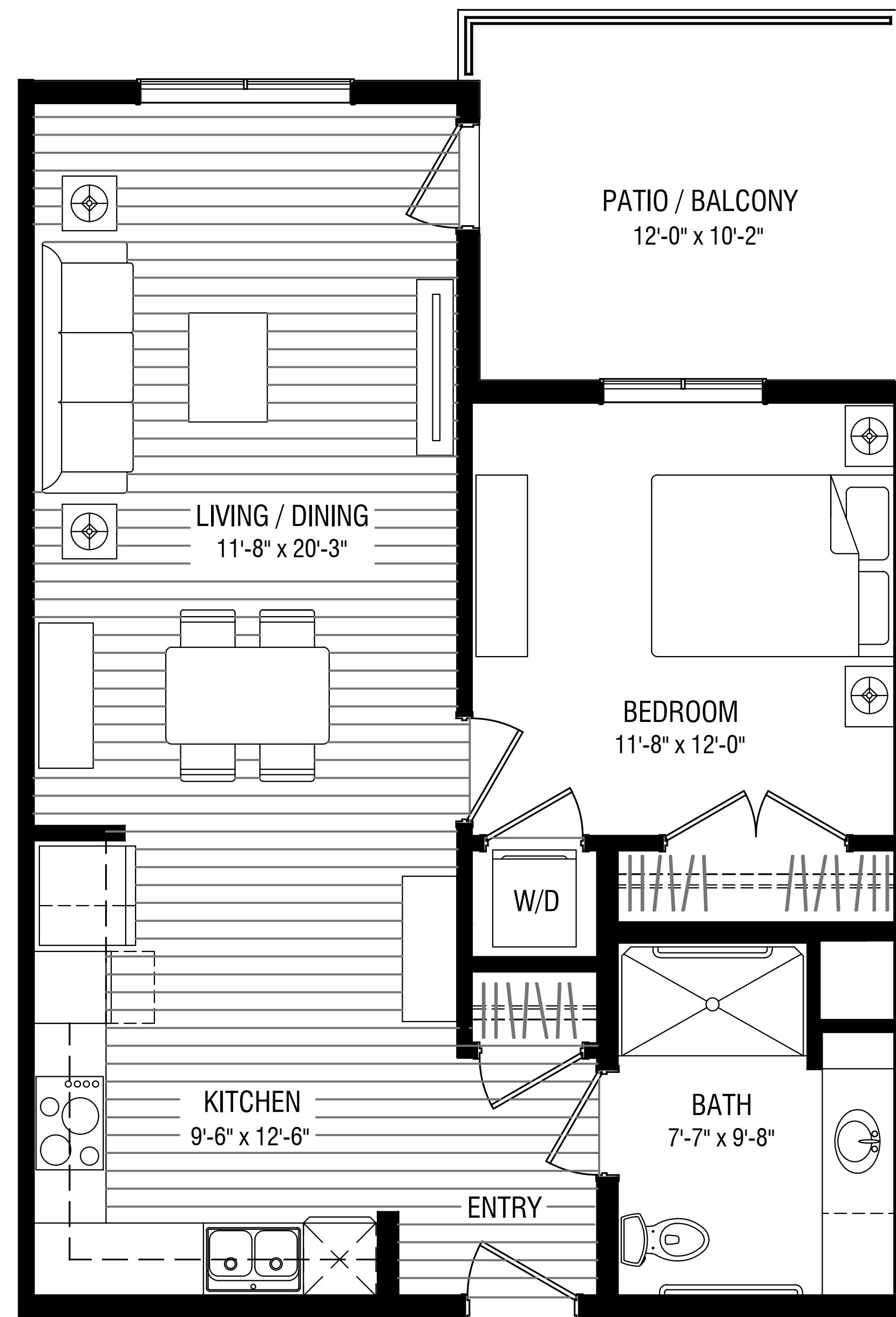
PLAN : SUITE TYPE B (AREA = 737 sq.ft.) SCALE : 1/8" = 1'-0"
