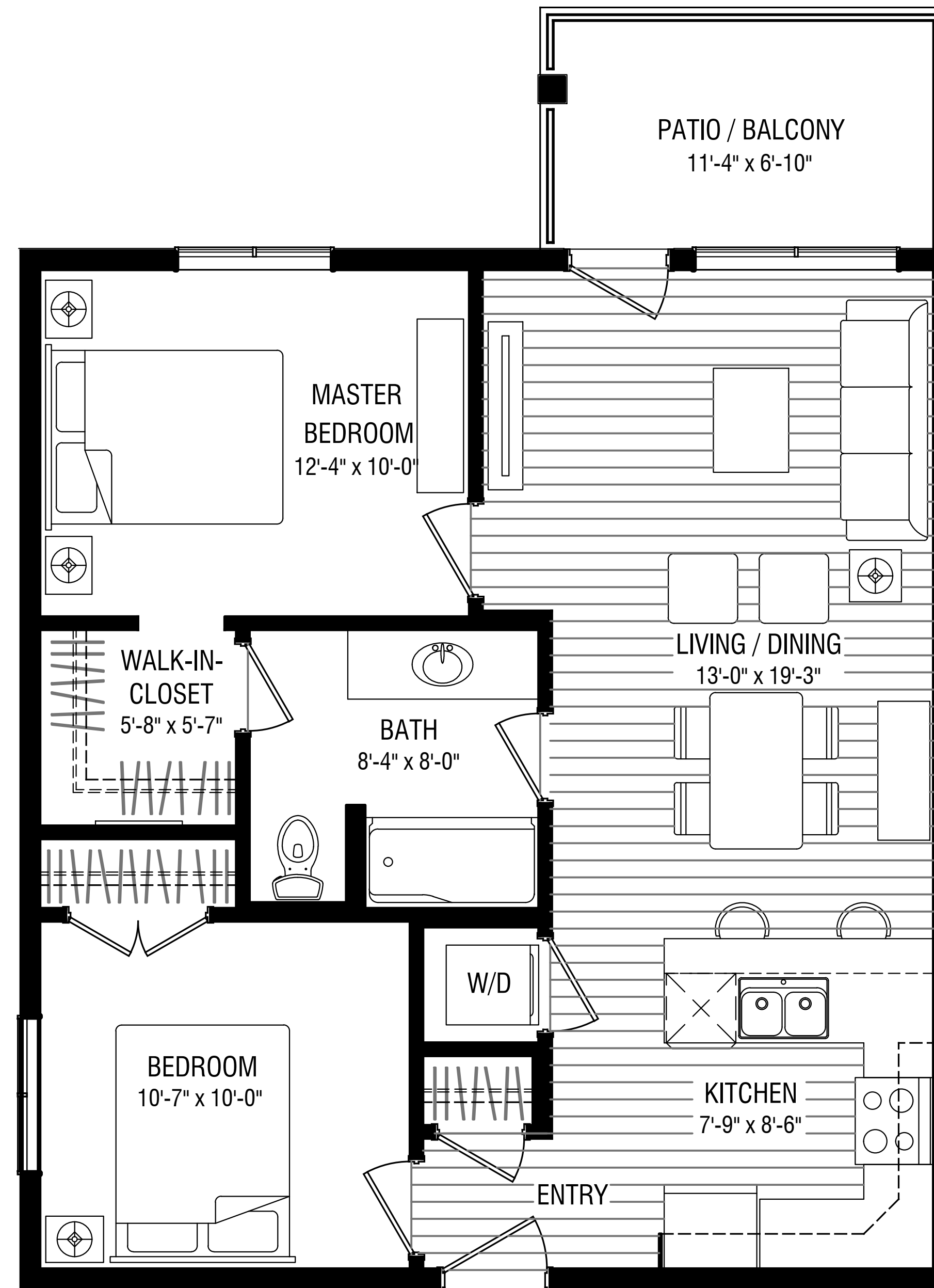
PLAN : SUITE TYPE D (AREA = 800 sq.ft.) SCALE : 1/8" = 1'-0"
