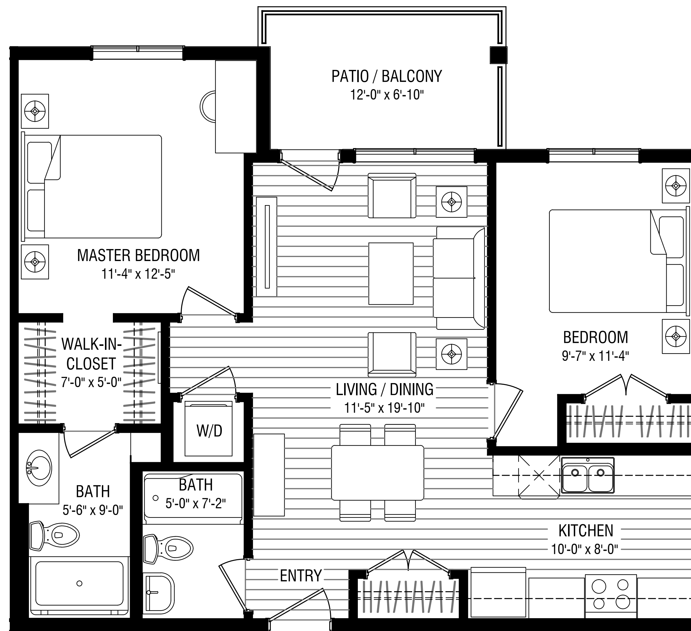
PLAN : SUITE TYPE E (AREA = 854 sq.ft.) SCALE : 1/8" = 1'-0"
