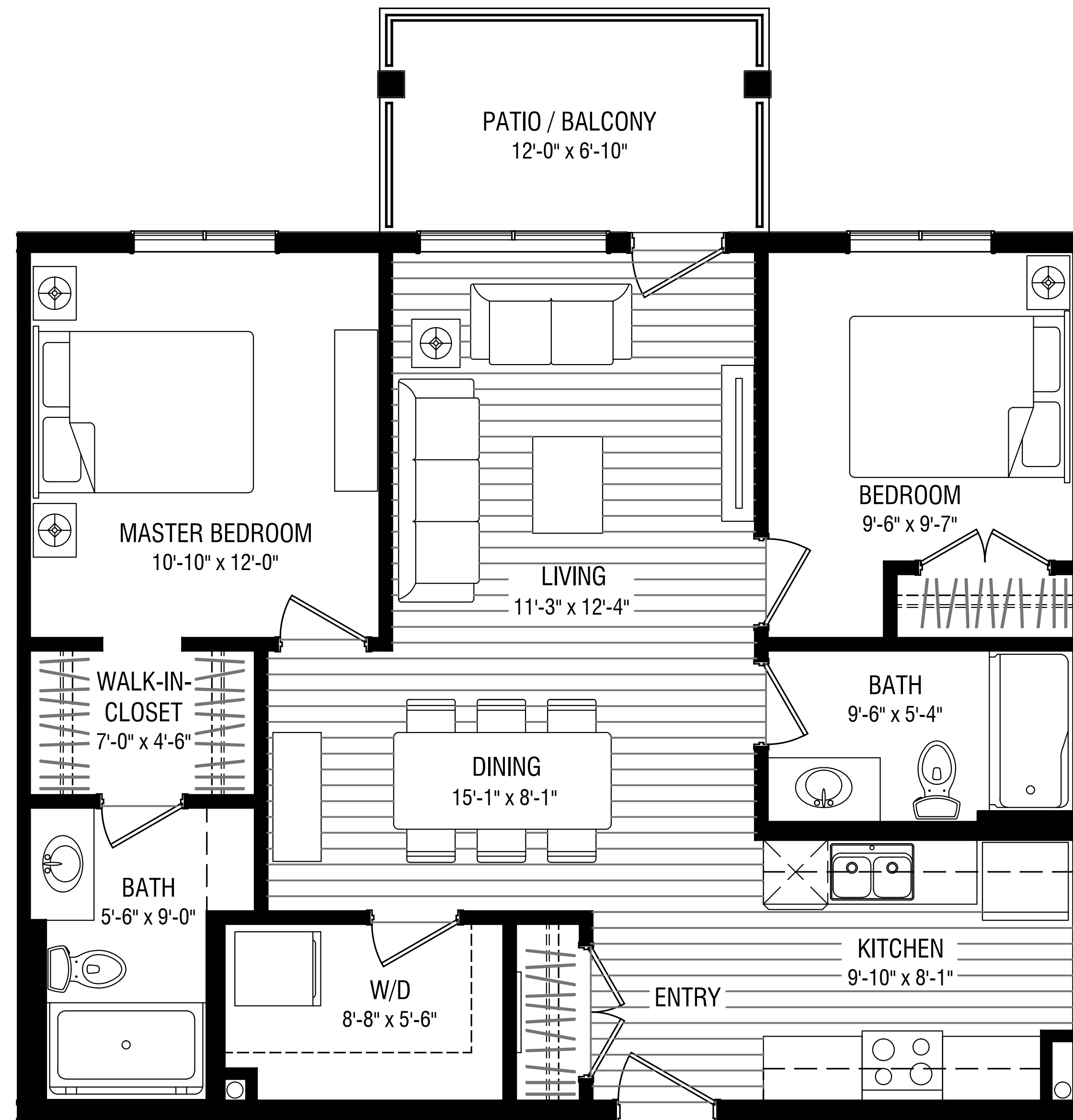
PLAN : SUITE TYPE F (AREA = 914 sq.ft.) SCALE : 1/8" = 1'-0"
